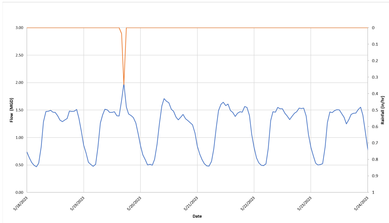
CHART 3-3 KORREDMO83 AND KORREDMO146 RAIN GAUGE HOURLY INTENSITY (FLOW VS. TIME, METER MH04C002)
