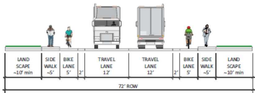
Figure 3: Industrial Street Typical Section
