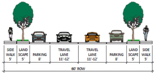
Figure 4: Minor Collector Typical Section
