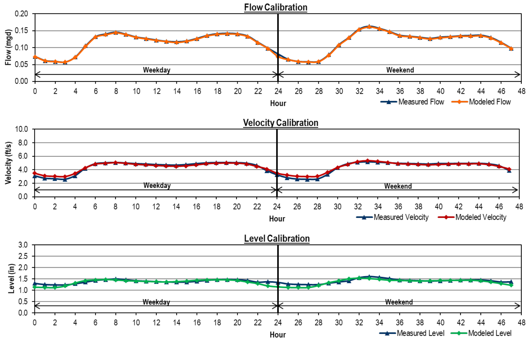
Figure 1.6 Example Diurnal Pattern (MH04C042)
