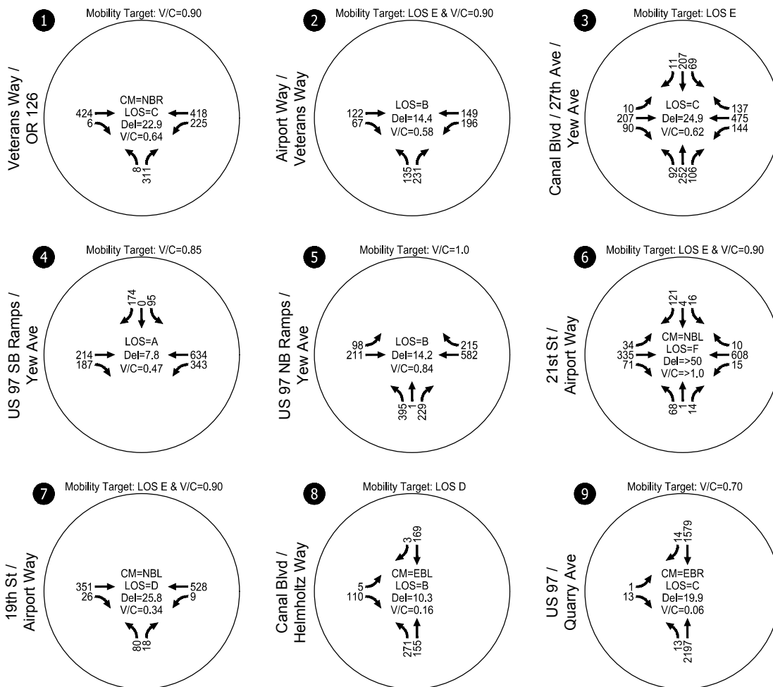
Existing Traffic Conditions 2023 PM Peak Hour Redmond, OR
