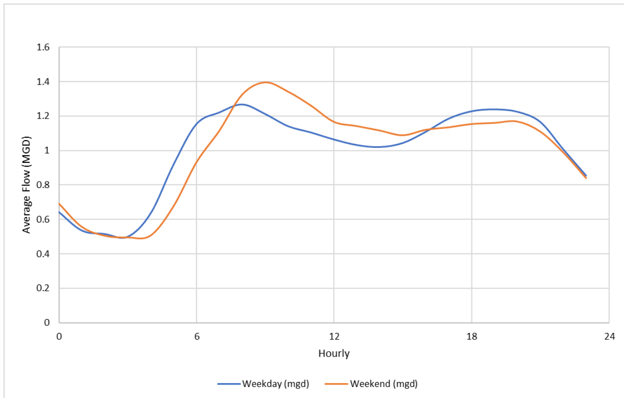
CHART 3-1 TYPICAL WEEKDAY VERSUS WEEKEND DRY WEATHER FLOW VARIATION (METER MH04C042 DIURNAL PATTERN)
