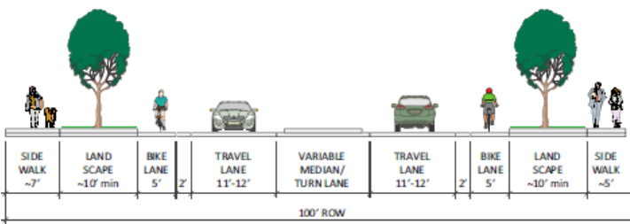
Figure 6: Minor Arterial Typical Section
