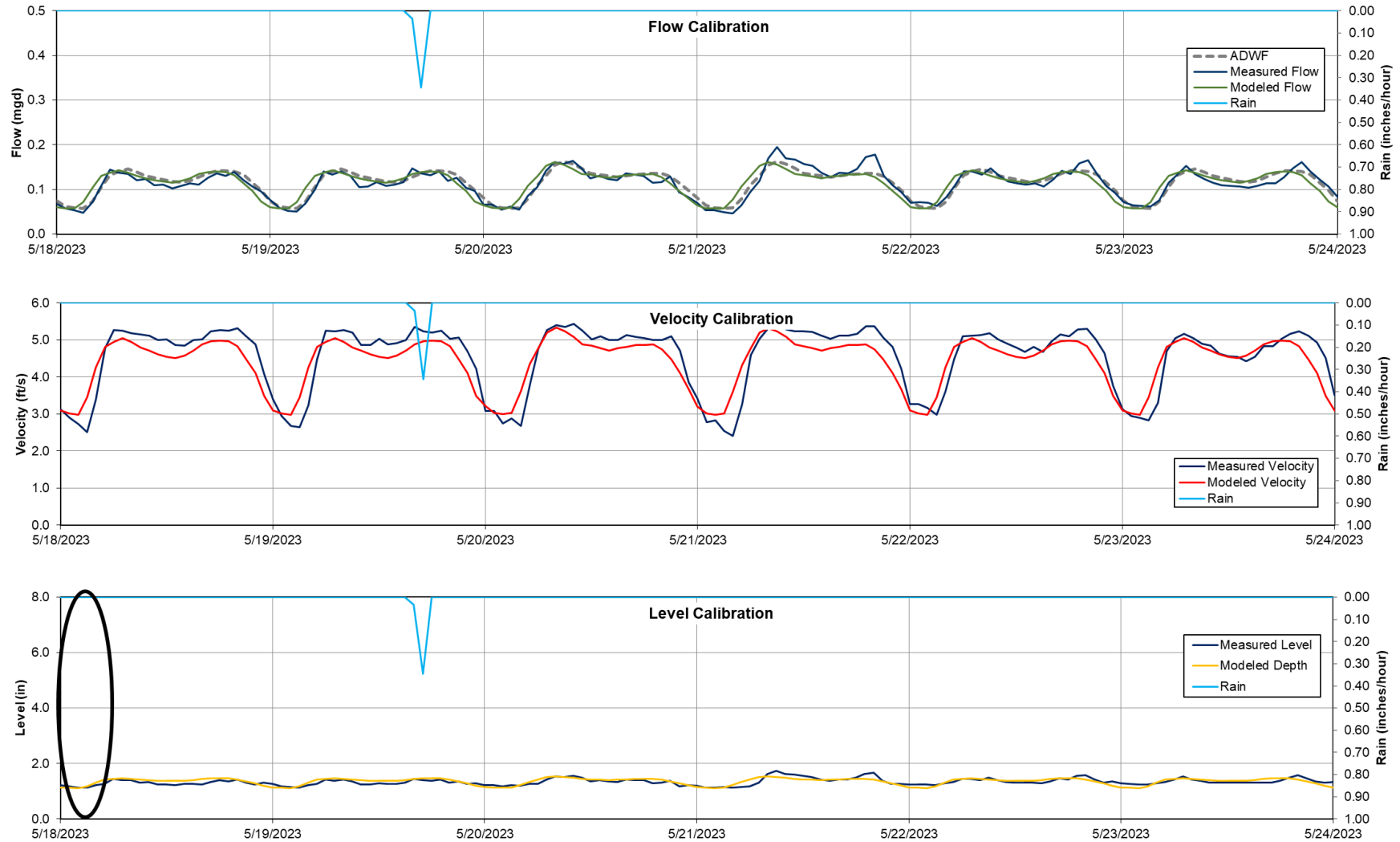
Figure 1.7 Example of Wet Weather Calibration - Meter MH04C042
