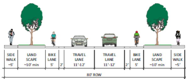
Figure 5: Major Collector Typical Section
