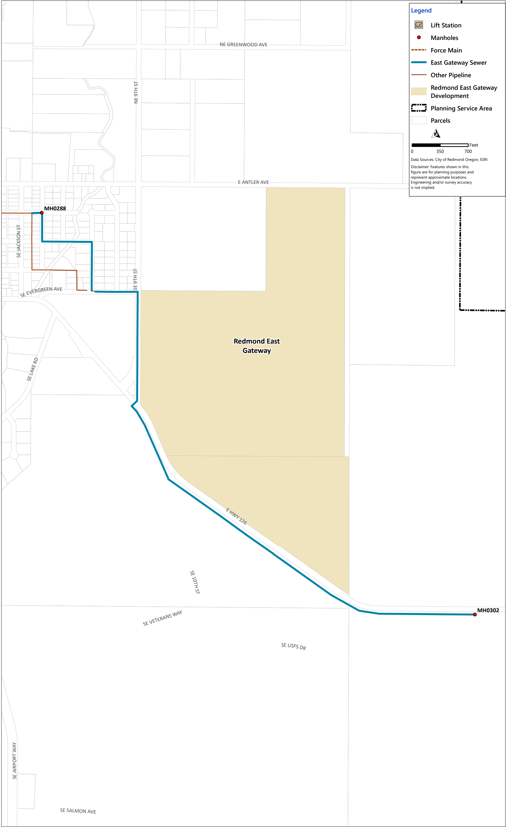
Figure 3.1 Planning Service Area and East Gateway Manhole Flow Allocation CITY OF REDMOND WASTEWATER COLLECTION SYSTEM MASTER PLAN UPDATE
