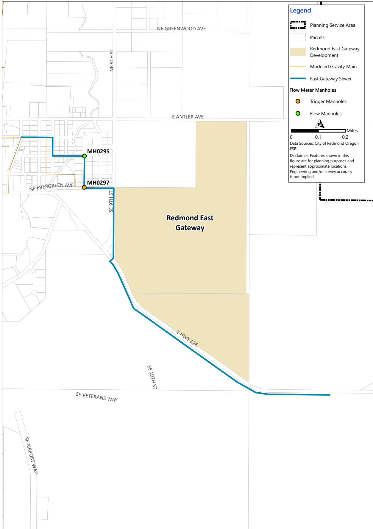
Figure 3.4 East Gateway Flow Monitoring Recommendation CITY OF REDMOND WASTEWATER COLLECTION SYSTEM MASTER PLAN UPDATE
