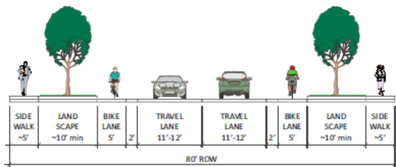
Figure 5: Major Collector Typical Section
