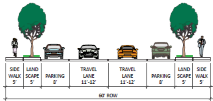
Figure 4: Minor Collector Typical Section
