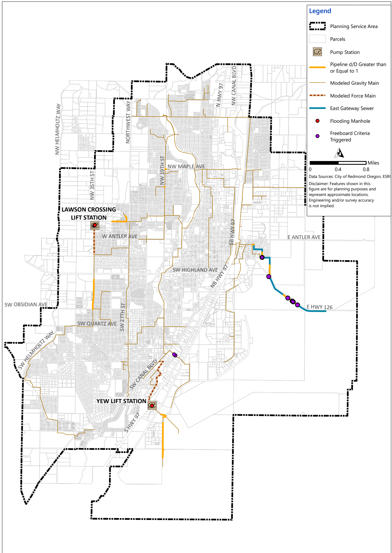
Figure 3.3 Build-out with HB 2001 Incorporating Developers' Flow Assumption Results CITY OF REDMOND WASTEWATER COLLECTION SYSTEM MASTER PLAN UPDATE
