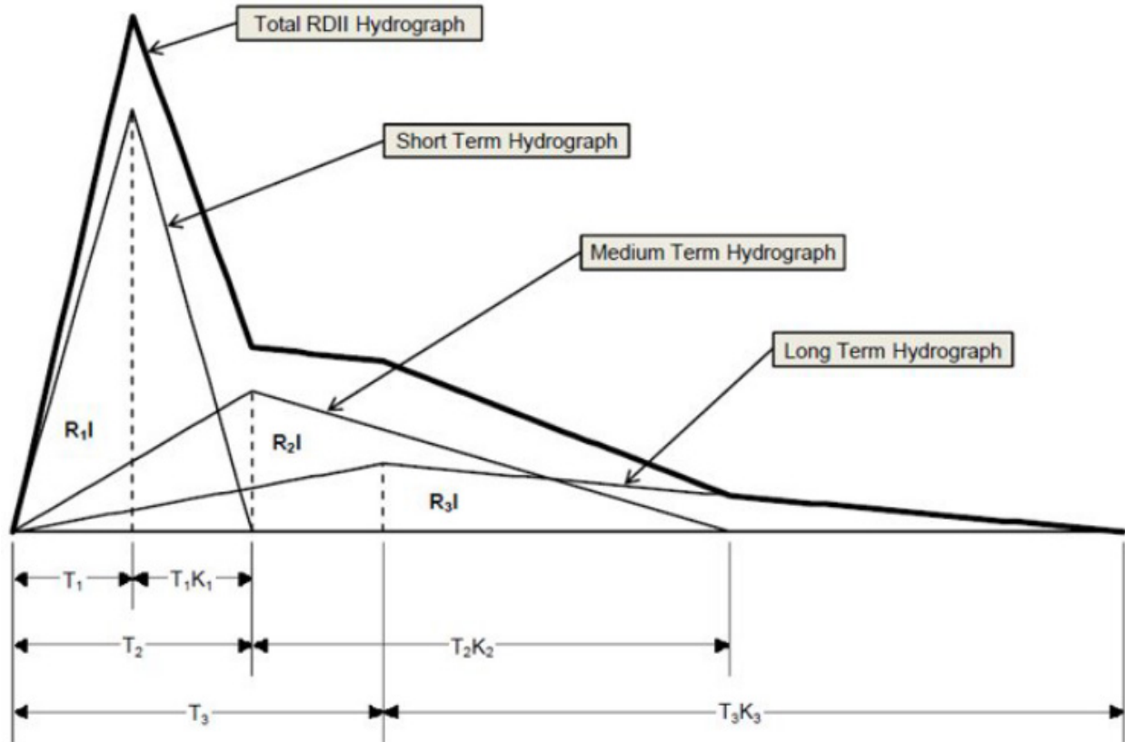
Figure 1.4 RTK Unit Hydrograph Description
