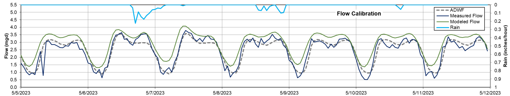
Figure 1.8 Verification of Wet Weather Calibration - WPCF
