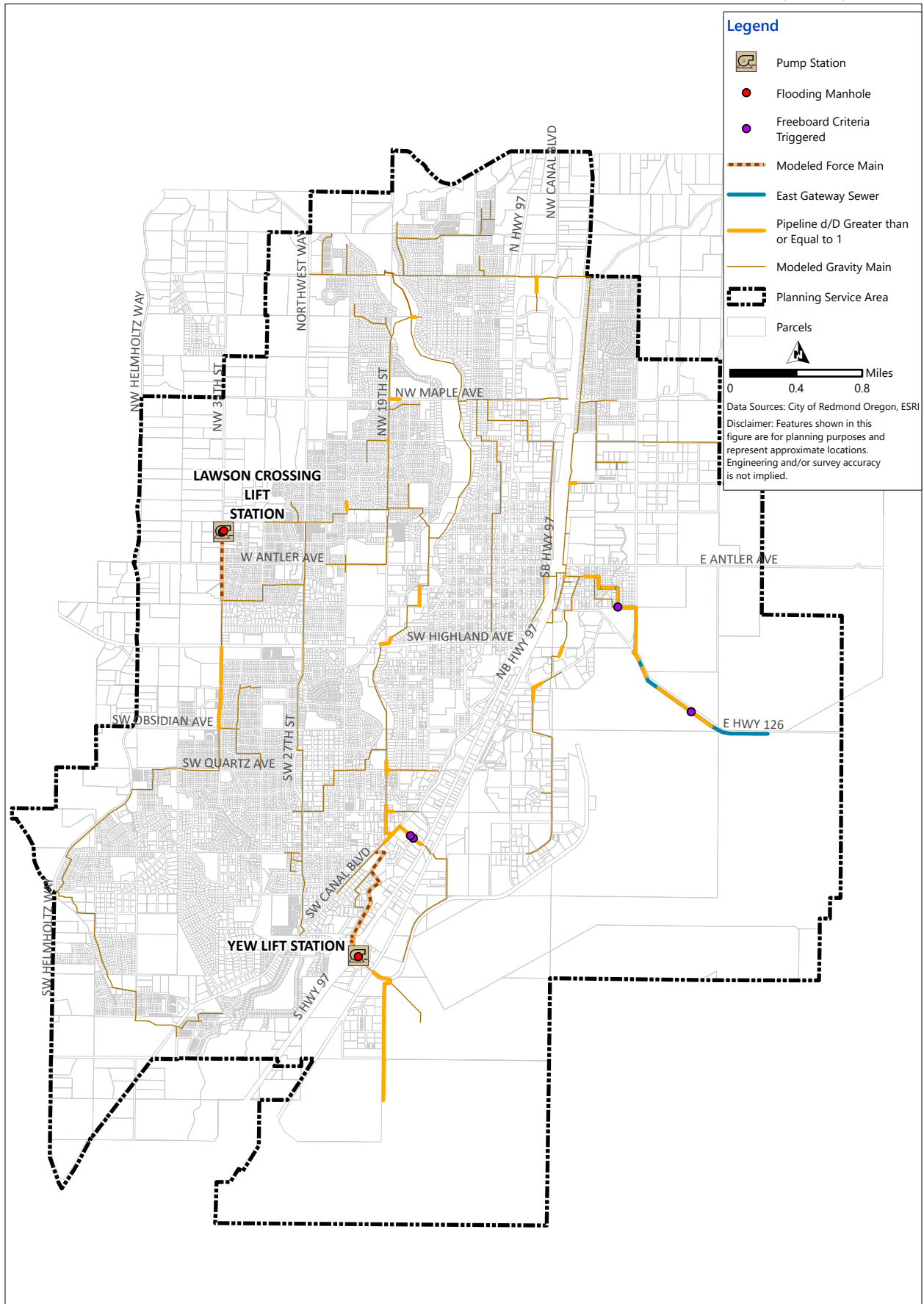
Figure 3.2 Buildout System with HB2001 Results
