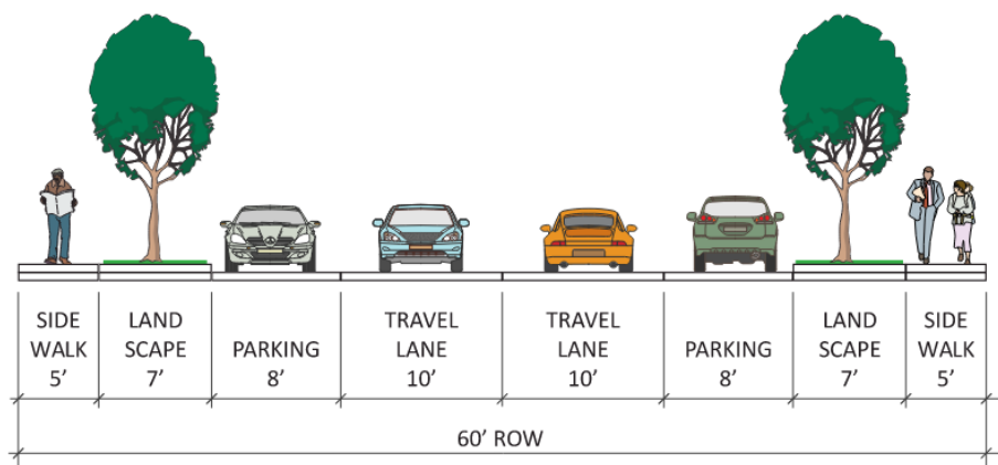
Figure 2: Standard Local Residential Typical Section
