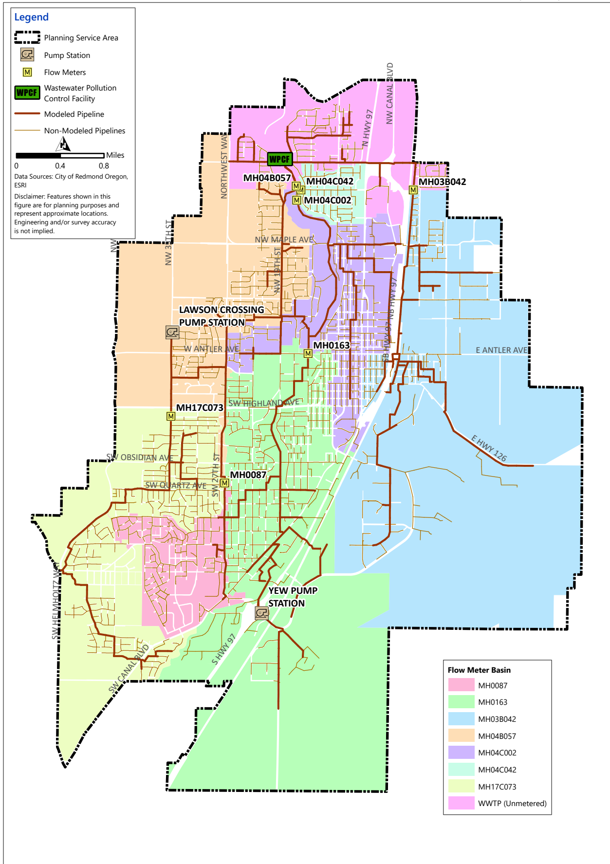
Figure 1.2 City of Redmond's Hydraulic Model CITY OF REDMOND WASTEWATER COLLECTION SYSTEM MASTER PLAN UPDATE
