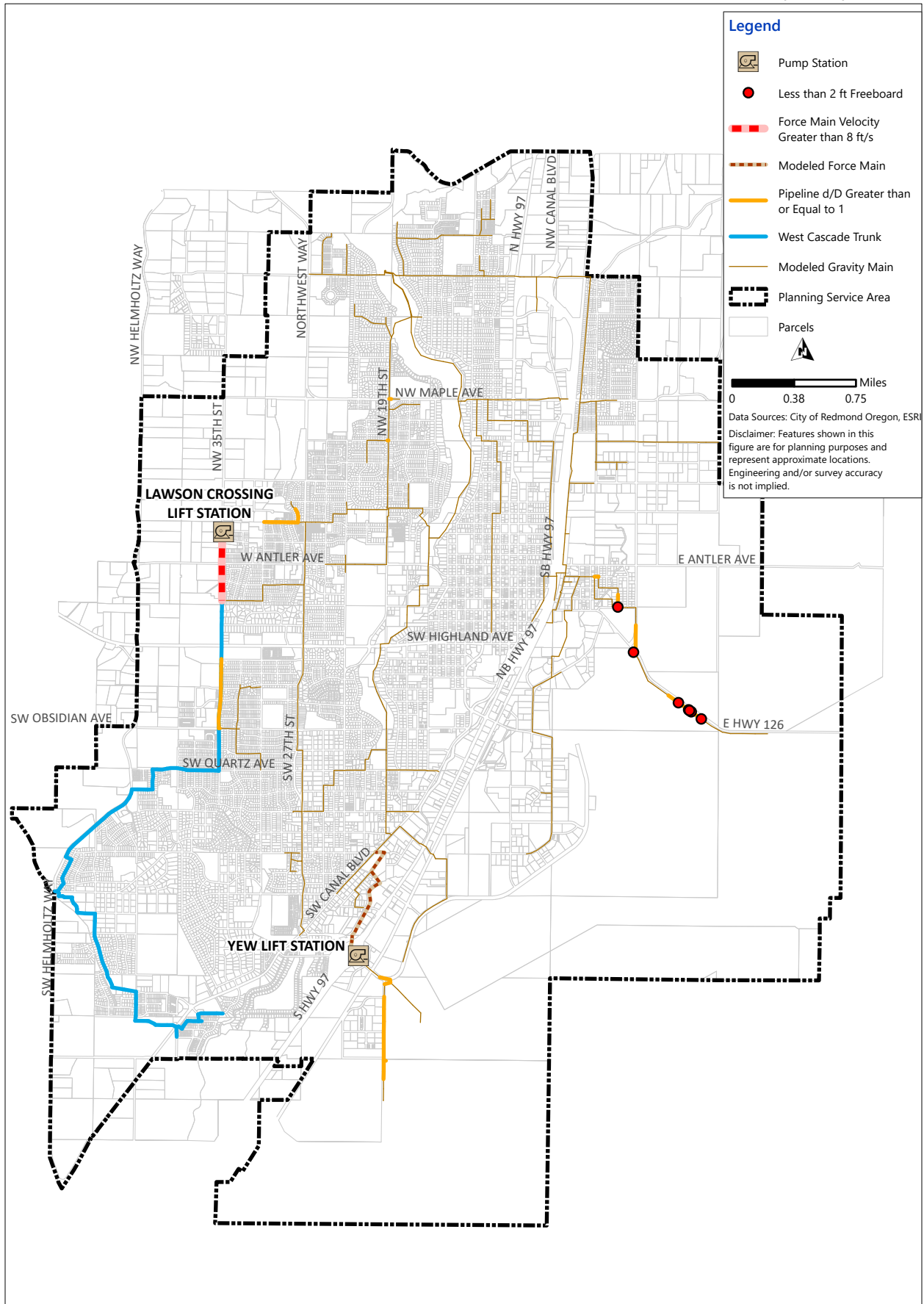
Figure 2.3 Build-out with HB 2001 Incorporating Developers' Flow Assumption Results CITY OF REDMOND WASTEWATER COLLECTION SYSTEM MASTER PLAN UPDATE
