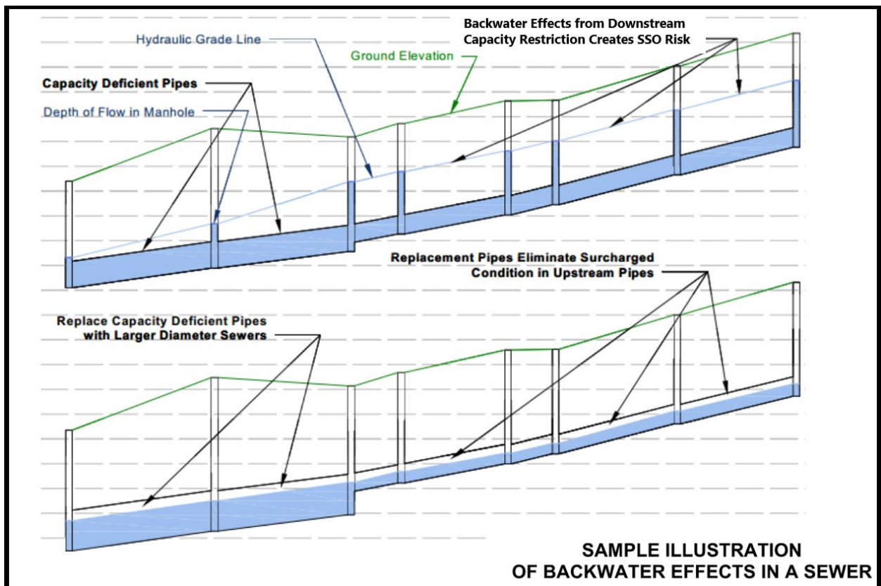
Figure 5-1 Sample Illustration of Backwater Effects in a Sewer
