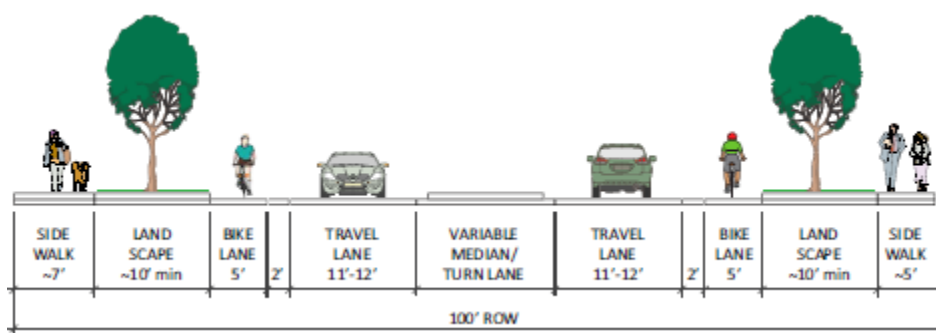
Figure 6: Minor Arterial Typical Section
