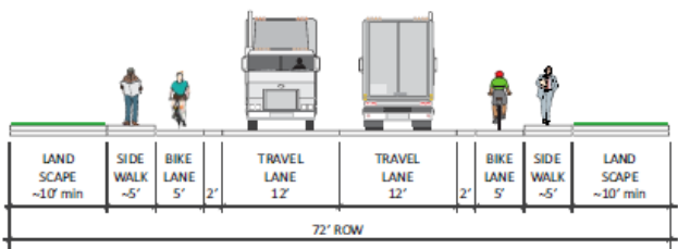
Figure 3: Industrial Street Typical Section
