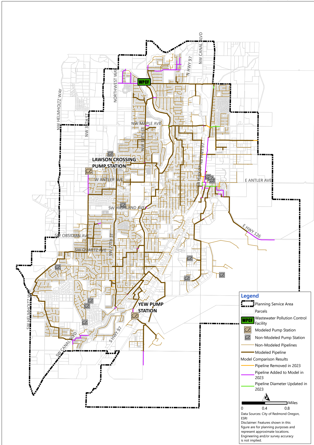
Figure 1.1 Model Comparison CITY OF REDMOND WASTEWATER COLLECTION SYSTEM MASTER PLAN UPDATE
