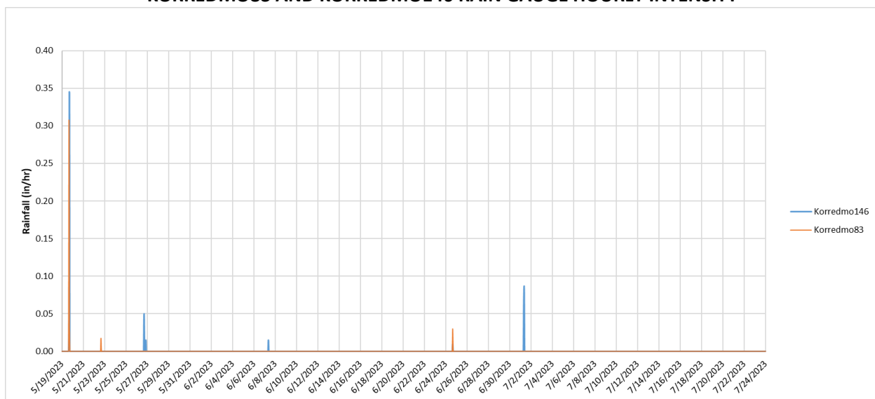
CHART 3-2 KORREDMO83 AND KORREDMO146 RAIN GAUGE HOURLY INTENSITY
