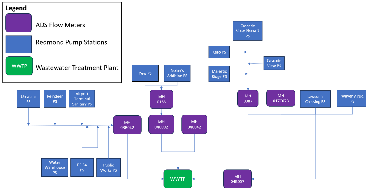
Figure 3-3 Flow Monitoring Schematic
