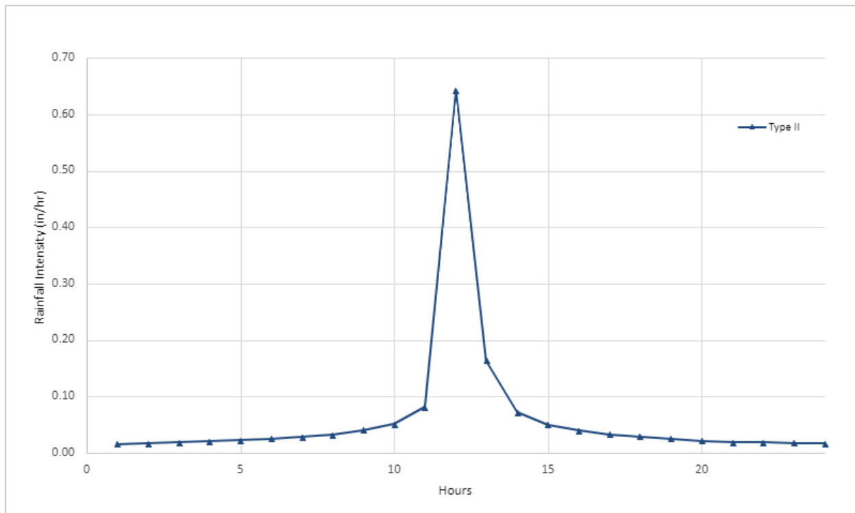
CHART 3-5 DESIGN STORM HYETOGRAPH (NOAA/SCS - 10-YR, 24-HR DESIGN STORM)
