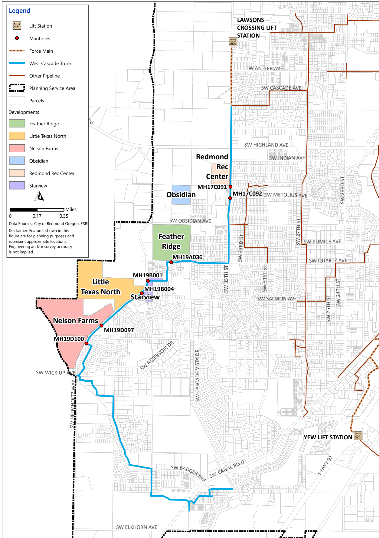
Figure 2.2 Overview Location of Developers' Manhole Flow Allocation CITY OF REDMOND WASTEWATER COLLECTION SYSTEM MASTER PLAN UPDATE
